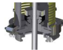
Mechanical Seal Cutaway
